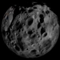
Phoebe
