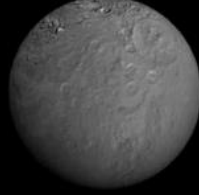
Rhea
