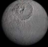
Tethys
